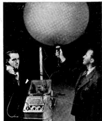
Joseph McDonald and Donald Kolb (holding balloon) are the Radiomarine engineers who developed and perfected this lifeboat radio. Here is the balloon that is inflated with helium—sending up the antenna. At left is the "miniature broadcasting station" and "telephone."
